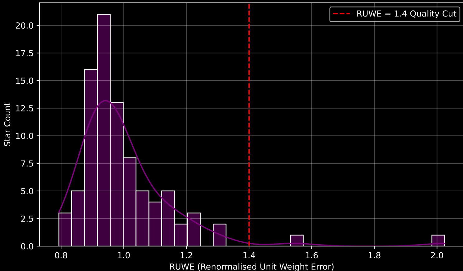
GAPOGEE DR17 Field [315-02-O] RUWE Distribution (n= 89)
