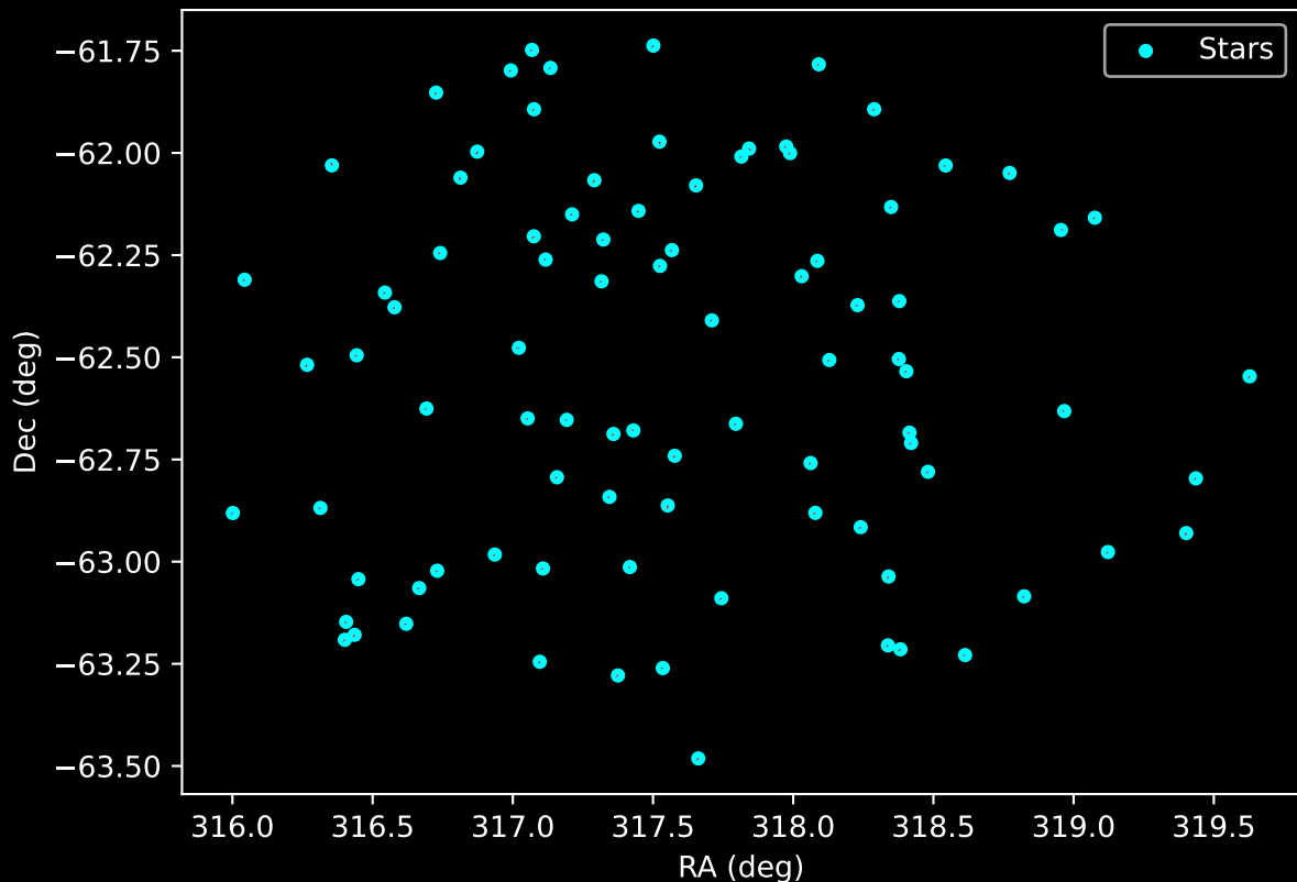
APOGEE DR17 Field: [315-02-O] Proper Motion Vectors for Gaia Star Field (n= 89)
