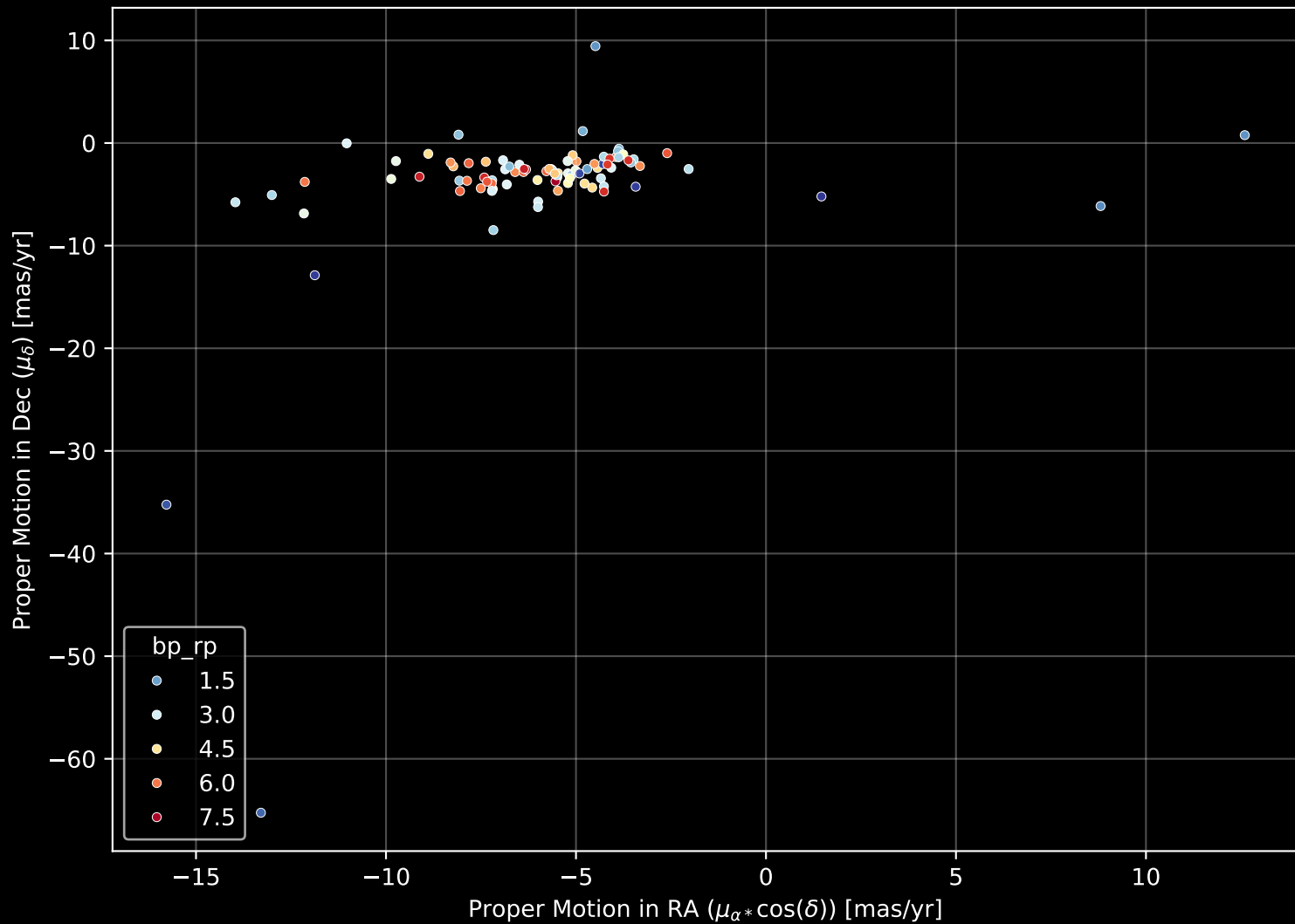
APOGEE DR17 Field: [315-02-O] Proper Motion Diagram (n= 89)
