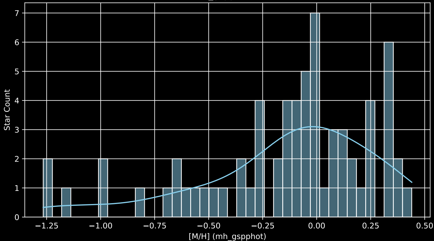
APOGEE DR17 Field: [315-02-O [M/H] (mh_gspphot) (n= 66)
