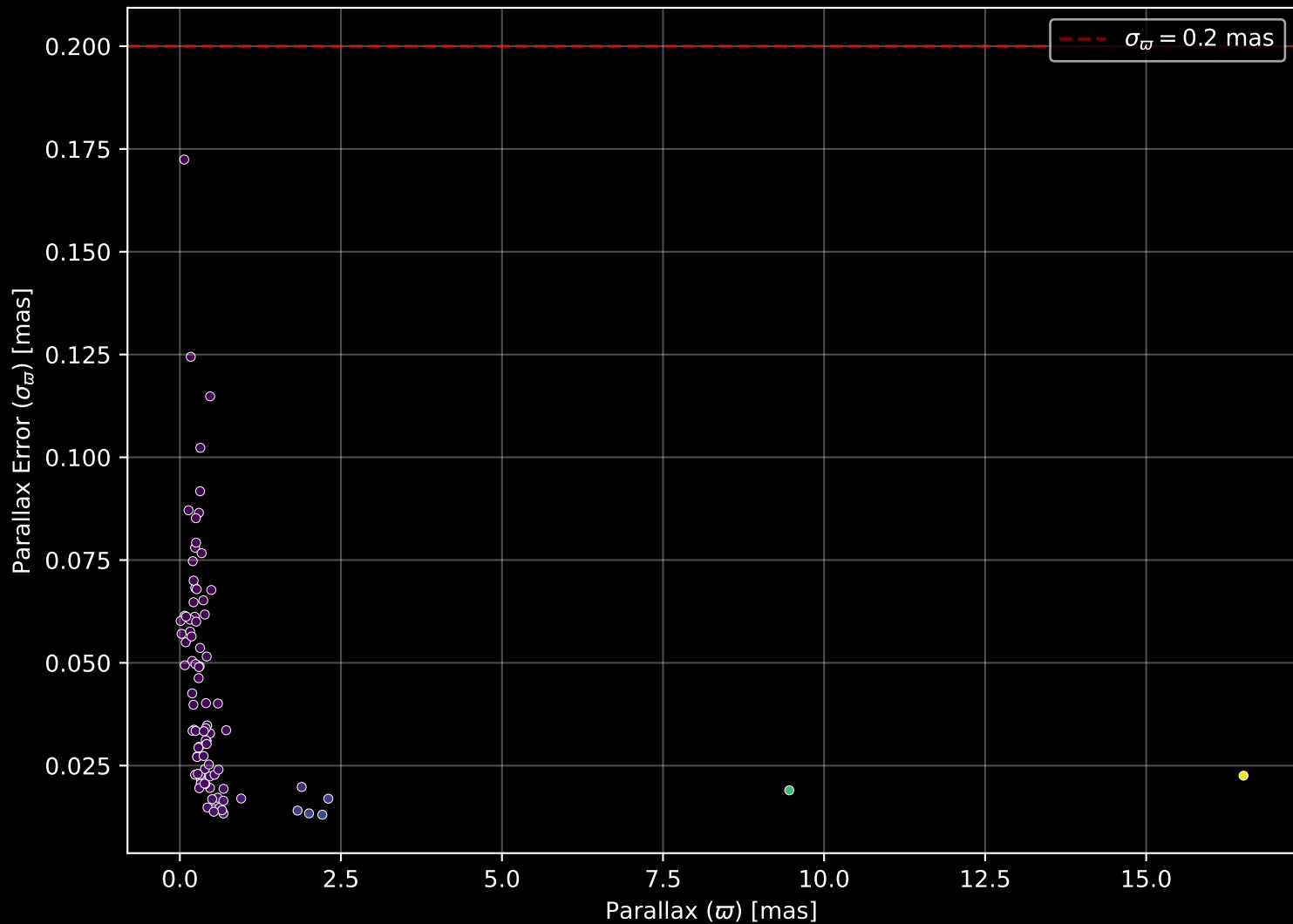
APOGEE DR17 Field: [315-02-O] Parallax Quality (n= 89)
