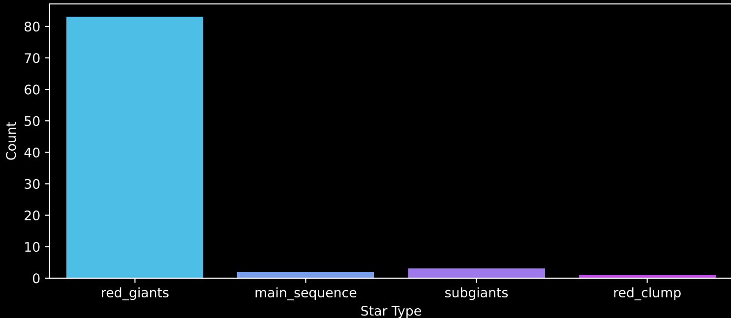
APOGEE DR17 Field: [315-02-O] Count plot of Star Type
