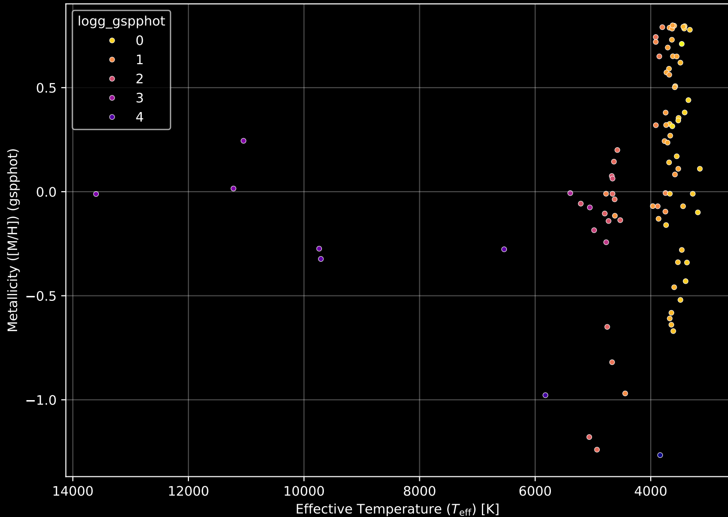
APOGEE DR17 Field: [315-02-O] Stellar Population Parameters (n= 89)
