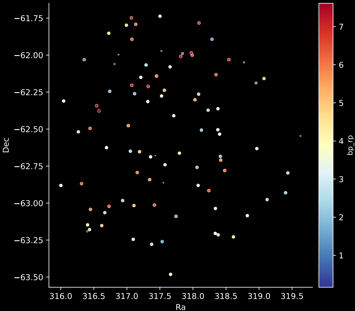
APOGEE DR17 Field: [315-02-O] Stars: 89
